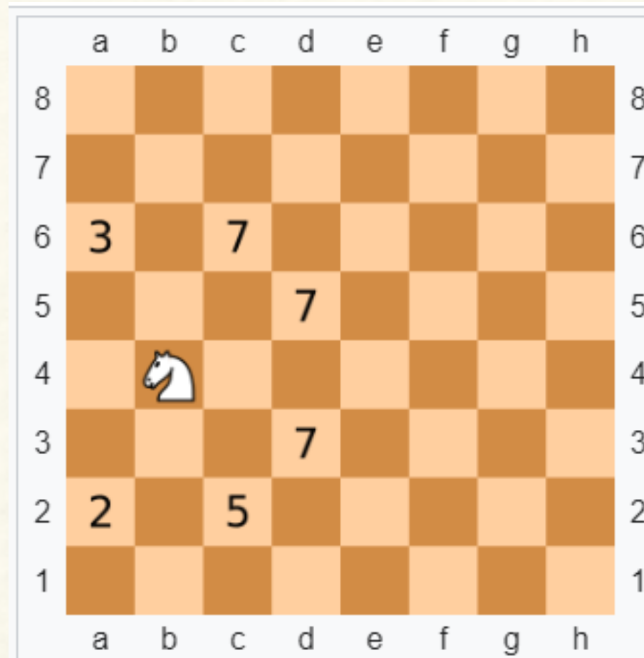
Warnsdorff's rule
