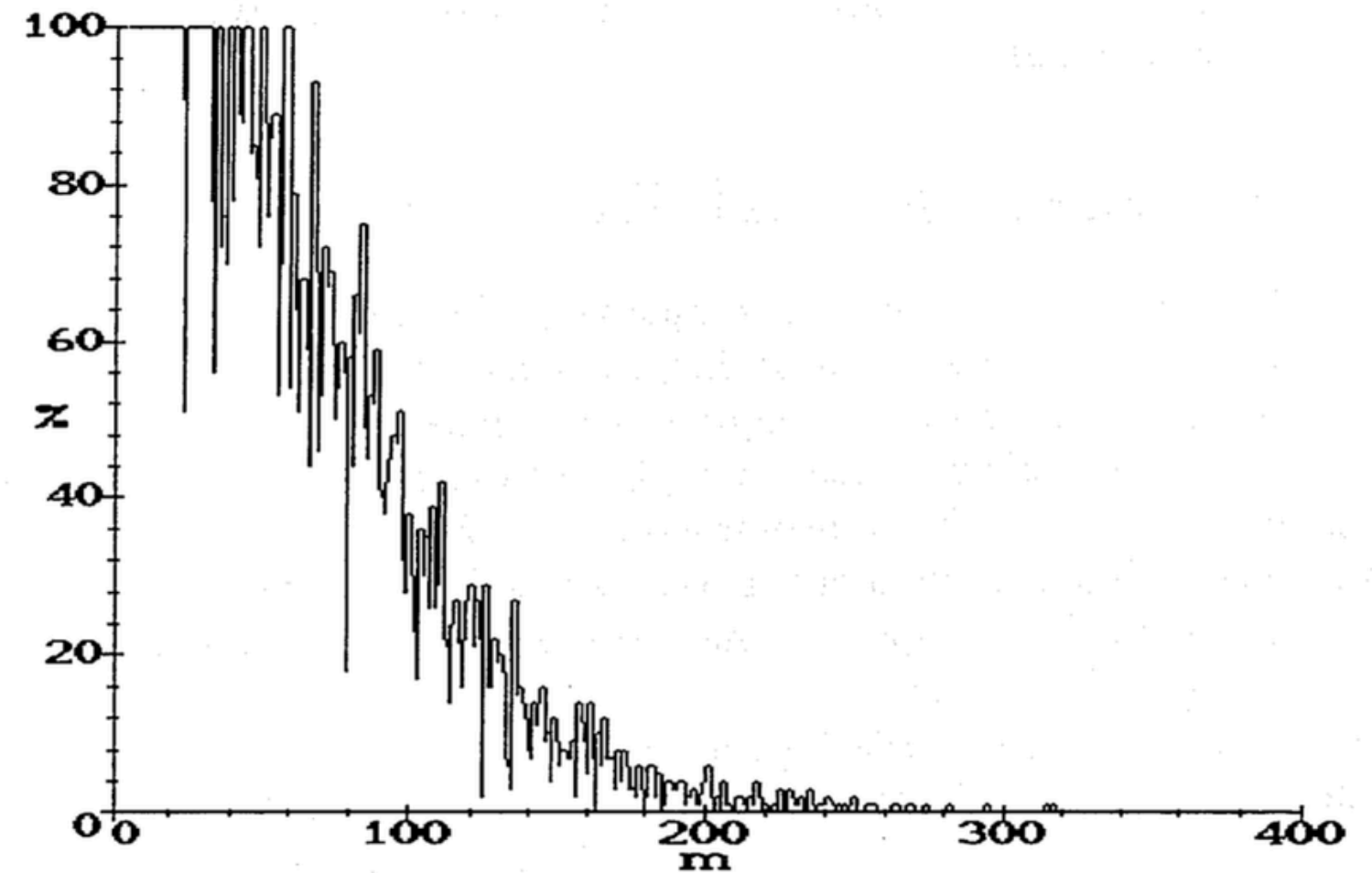
Figure 2: Success rate of random tiebreak rule.
