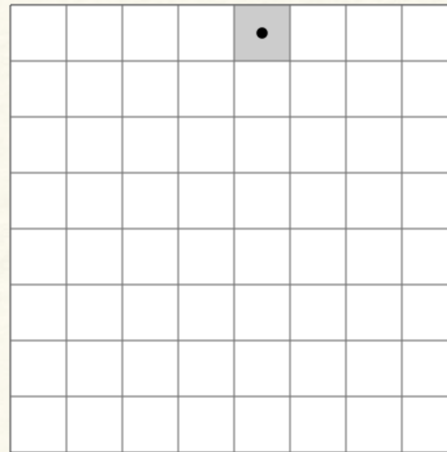
OPEN Knight's Tour
