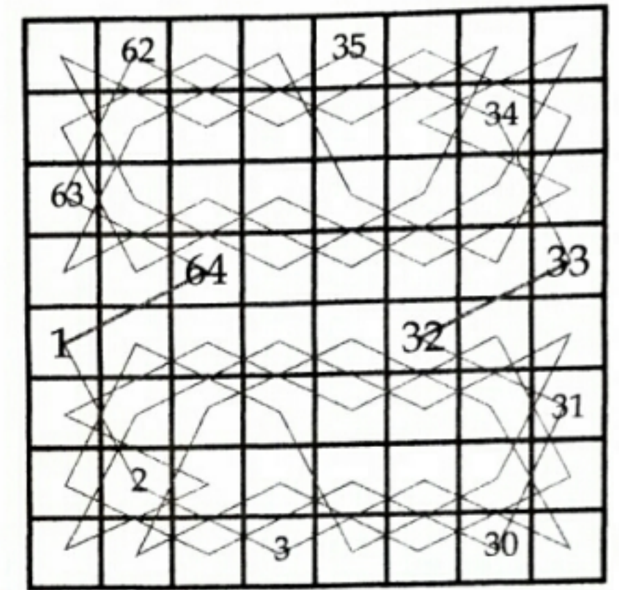
Figure 1: a knight's tour found by Euler
