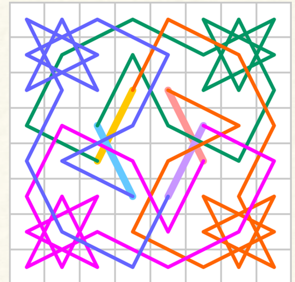
Figure 1: a knight's tour found by Euler
